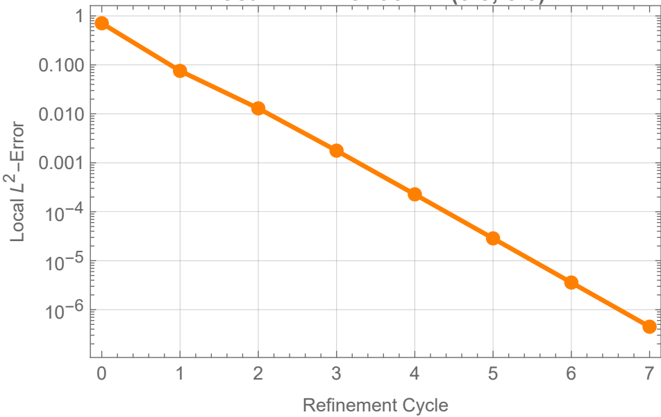
Local L^2 -Error at B = (0.5, 0.5)
